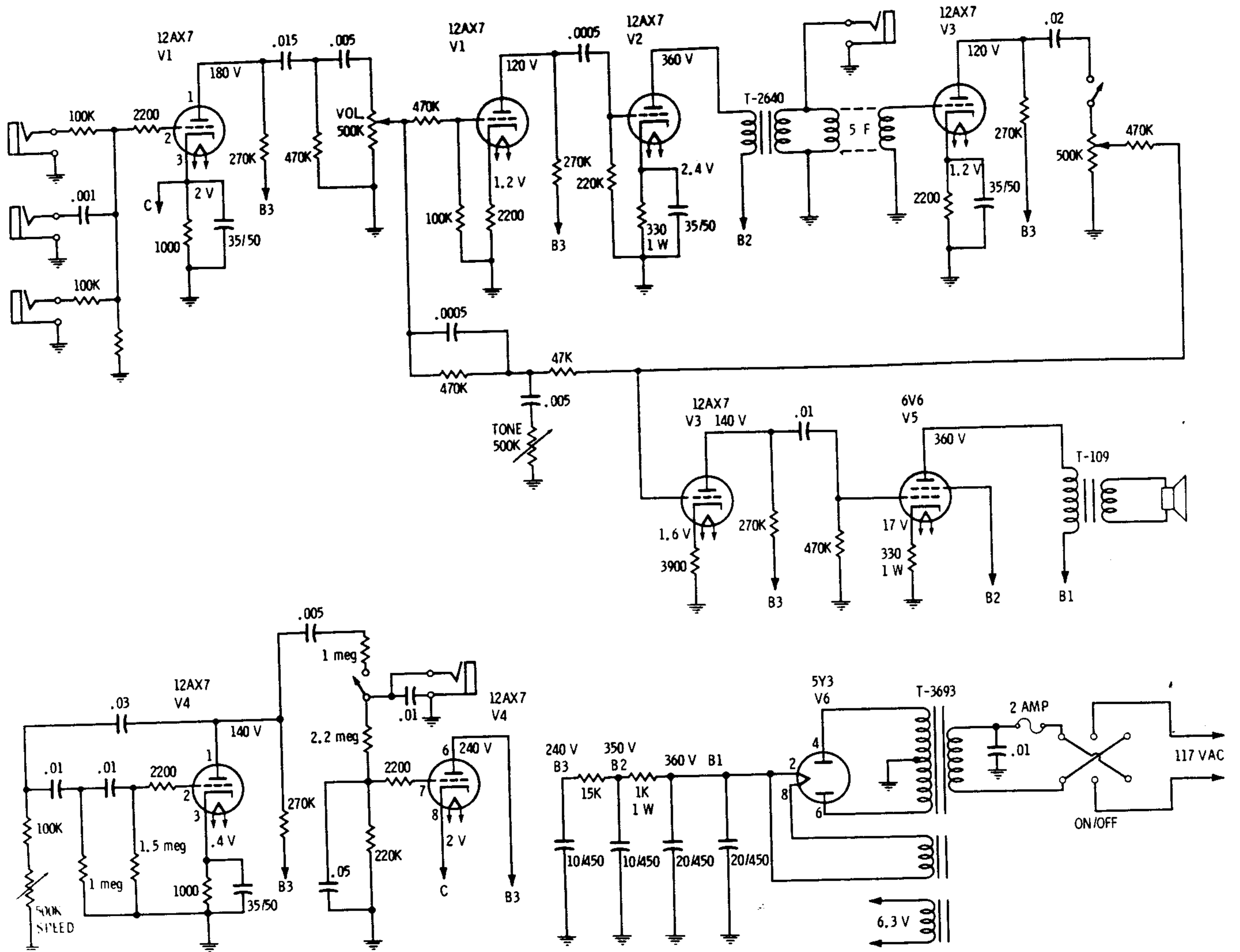
Gretsch Model G6152
